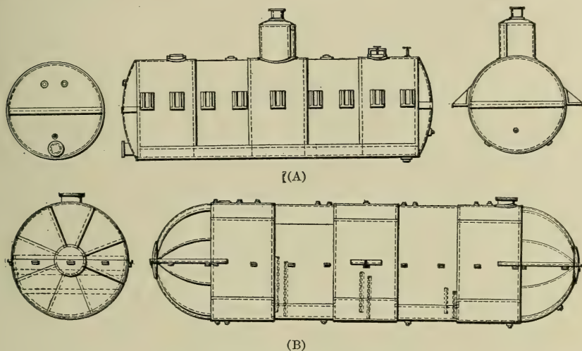
FIG. 105.—Horizontal Petroleum Stills.
